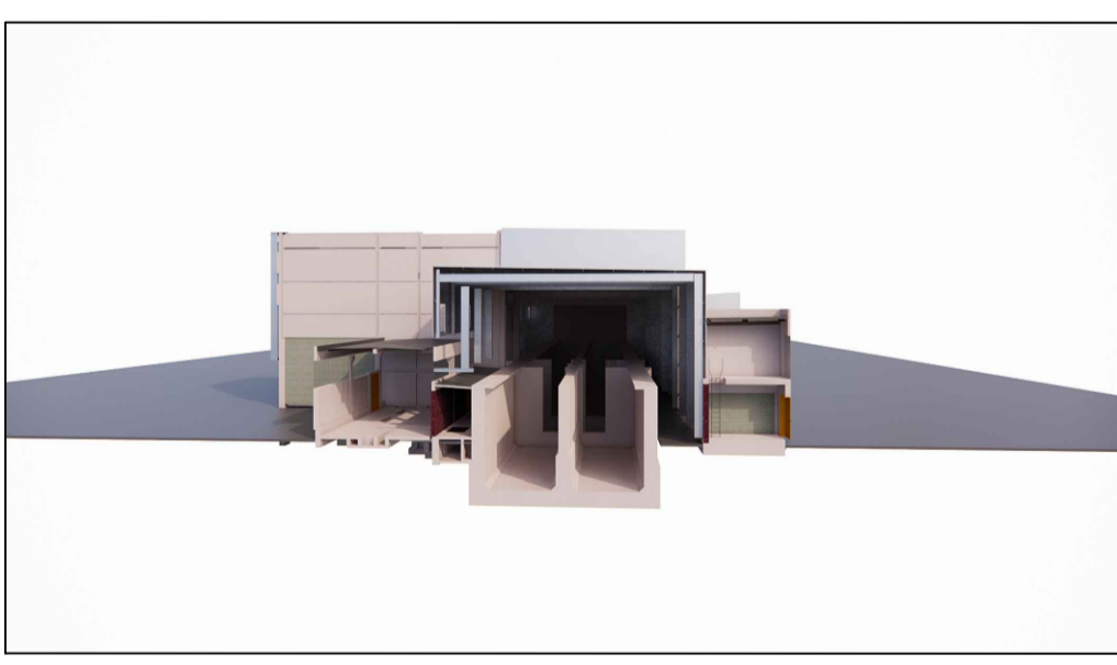
SECTION 15 (FACING NORTH)
